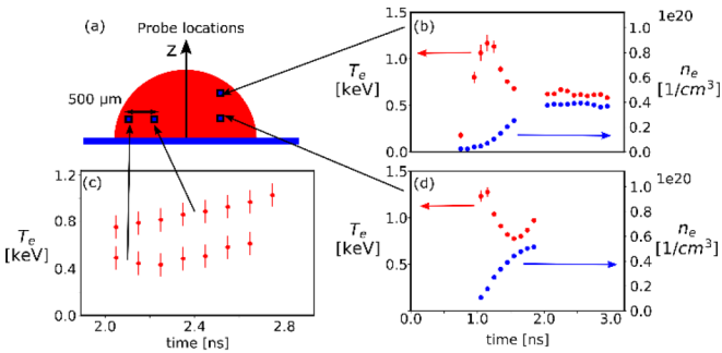
FIG. 5. Thomson scattering data at different locations in the plasma. The beam focus is \sim 800 \mu\text{m} in diameter. The three different measurement points (a single measurement point per shot) are laterally separated from the focus center by 1000, 1000, and 1500 \mu\text{m} and vertically separated from the foil surface by 500, 1000, and 500 \mu\text{m} , respectively. (b)–(d) Electron density (blue, right axis) and electron temperature (red, left axis) are extracted from the electron plasma wave contribution to the Thomson scattering spectrum. The temperature and density histories are collected in 1 ns streaks on separate shots; an example of evidence of shot-to-shot reproducibility can be seen in (b), where both the temperature and density traces are continuous despite the early time (0.8–1.8 ns) and late time (2.0–3.0 ns). (c) The measurement of temperature at two different locations, from which the temperature gradient scale length can be directly measured.
